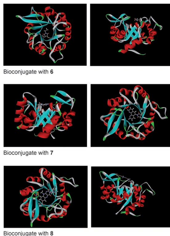
Figure 3. Bioconjugates made by treating mutant Cys9Ala/Asp11Cys with Michael acceptors 6 , 7 , and 8 . The putative structures were generated by manual docking of the respective ligands into the tHisF structure.
