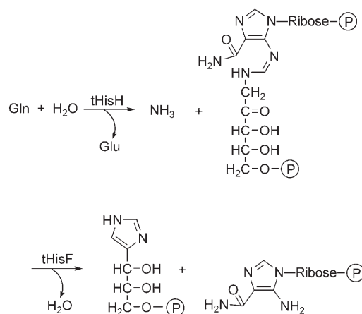
Scheme 1. Natural reaction of the bienzyme complex tHisH–tHisF. [12]
