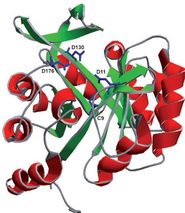
Figure 2. X-ray crystal structure of tHisF [12a,c] showing in blue the natural catalytic amino acids Asp11, Asp130, and Asp176, as well as Cys9.
