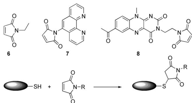
Scheme 2. Bioconjugation of the tHisF mutant Cys9Ala/Asp11Cys at position Cys11.
