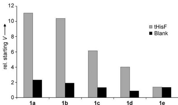
Figure 1. Relative activity of the tHisF-catalyzed hydrolysis of p -nitrophenyl esters 1a–e .
